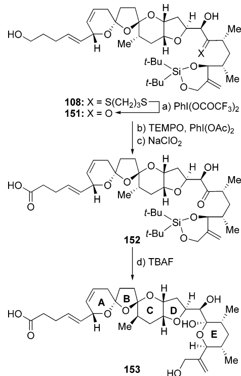
Scheme 13. Synthesis of Truncated ABCDE Azaspiracid-1 152 a
