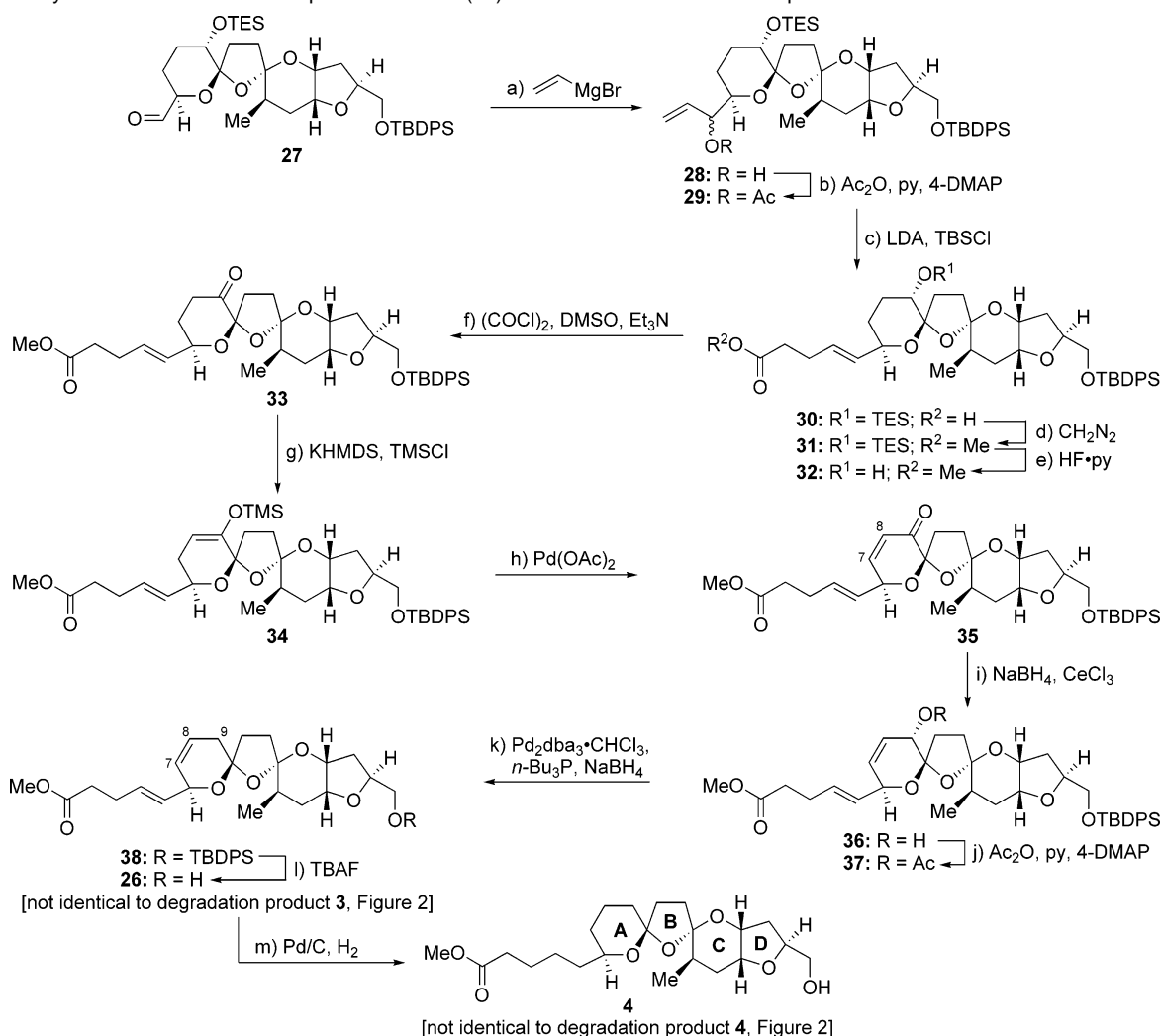
Scheme 4. Synthesis of the Second Proposed Structure ( 26 ) of the ABCD Domain of Azaspiracid-1 a
