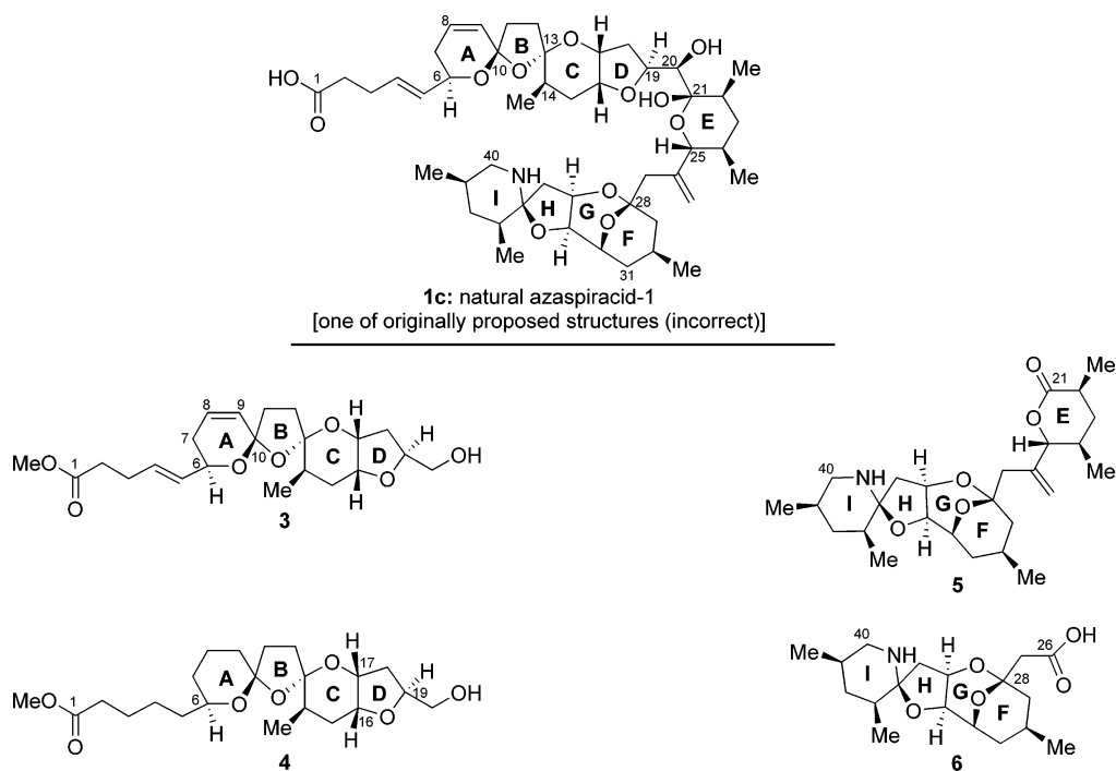
Figure 2. Proposed structures of fragments 3 – 6 obtained from degradation of natural azaspiracid-1 ( 1c ) by Satake et al.
