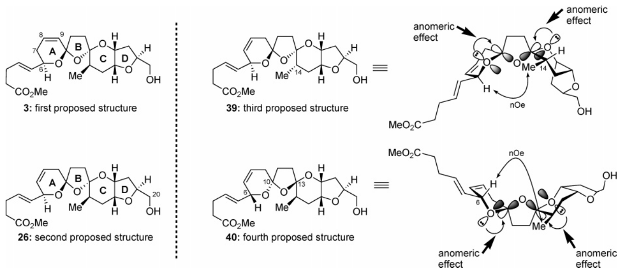
Figure 3. Third ( 39 ) and fourth ( 40 ) proposed structures for the ABCD domain of azaspiracid-1 with expected anomeric effects and nOes.
