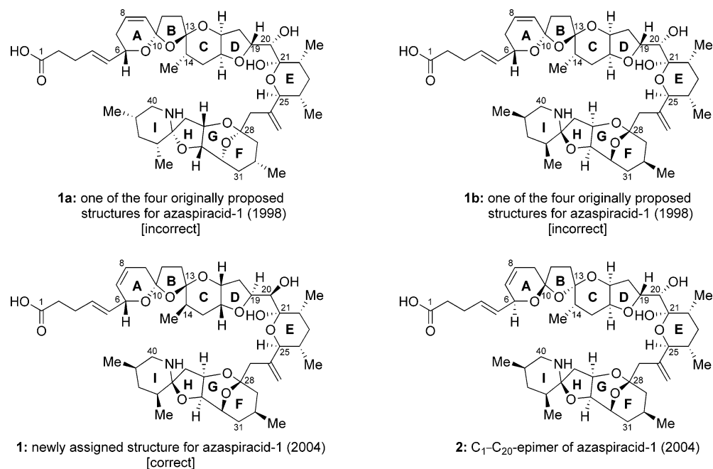
Figure 1. Two of the four originally proposed structures of azaspiracid-1 ( 1a and 1b ), proven to be incorrect, and structures of azaspiracid-1 ( 1 ) and its C 1 –C 20 epimer ( 2 ), proven to be correct by total synthesis.
