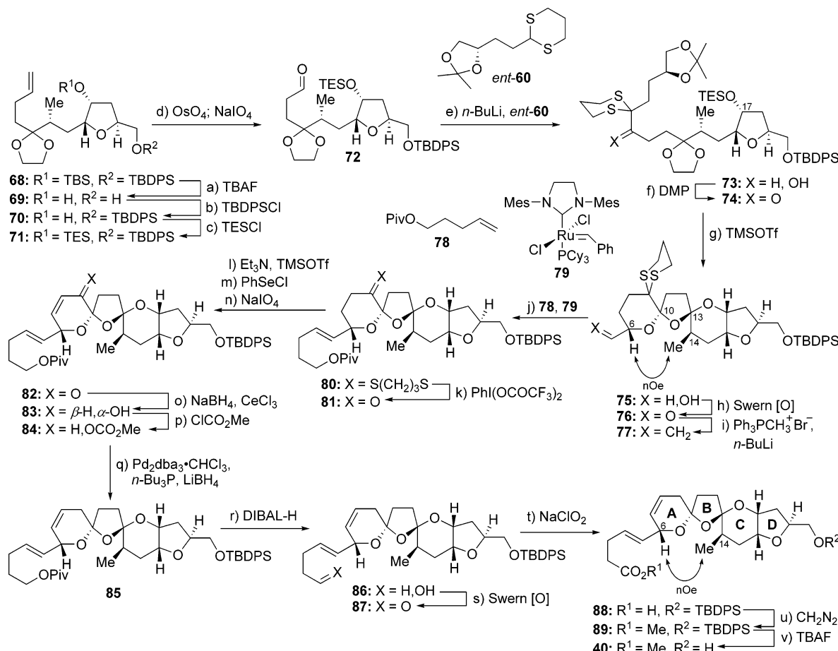
Scheme 7. Construction of the Fourth Proposed Structure ( 40 ) for the ABCD Domain of Azaspiracid-1 a
