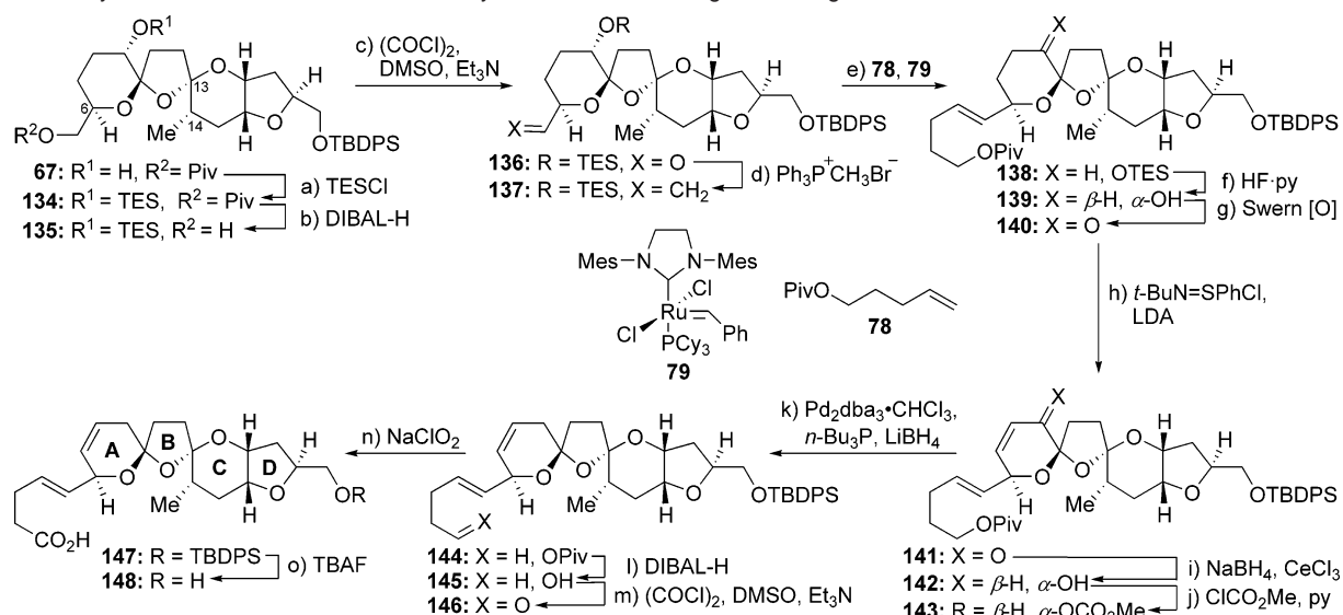
Scheme 11. Synthesis of Truncated ABCD Carboxylic Acid 148 for Biological Testing a
