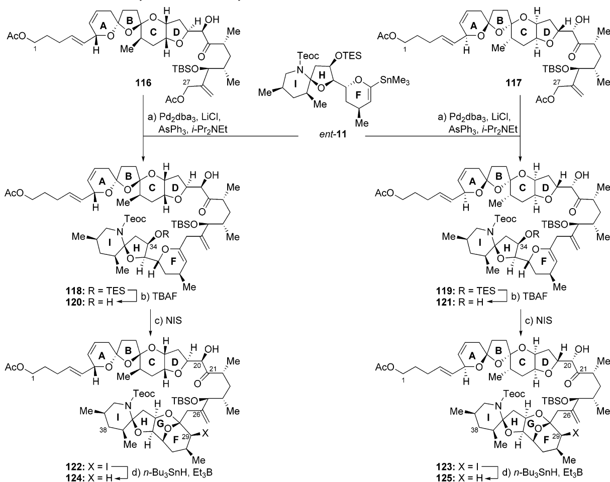
Scheme 9. Advancement to Octacyclic ABCD–FGHI Systems 124 and 125 a
