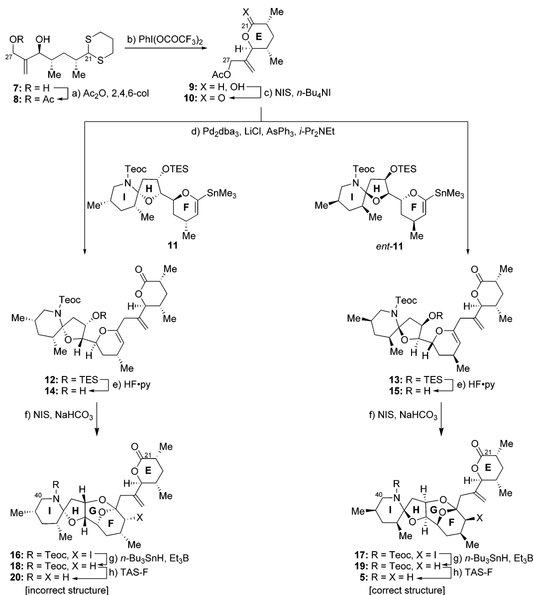
Scheme 1. Synthesis of C 21 –C 40 Lactones 5 and 20 and Determination of Relative and Absolute Stereochemistry within the EFGHI Domain a
