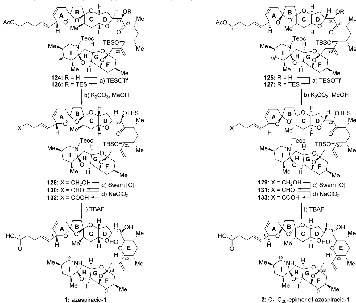
Scheme 10. Total Synthesis of Azaspiracid-1 ( 1 ) and Its C 1 –C 20 Epimer ( 2 ) a
