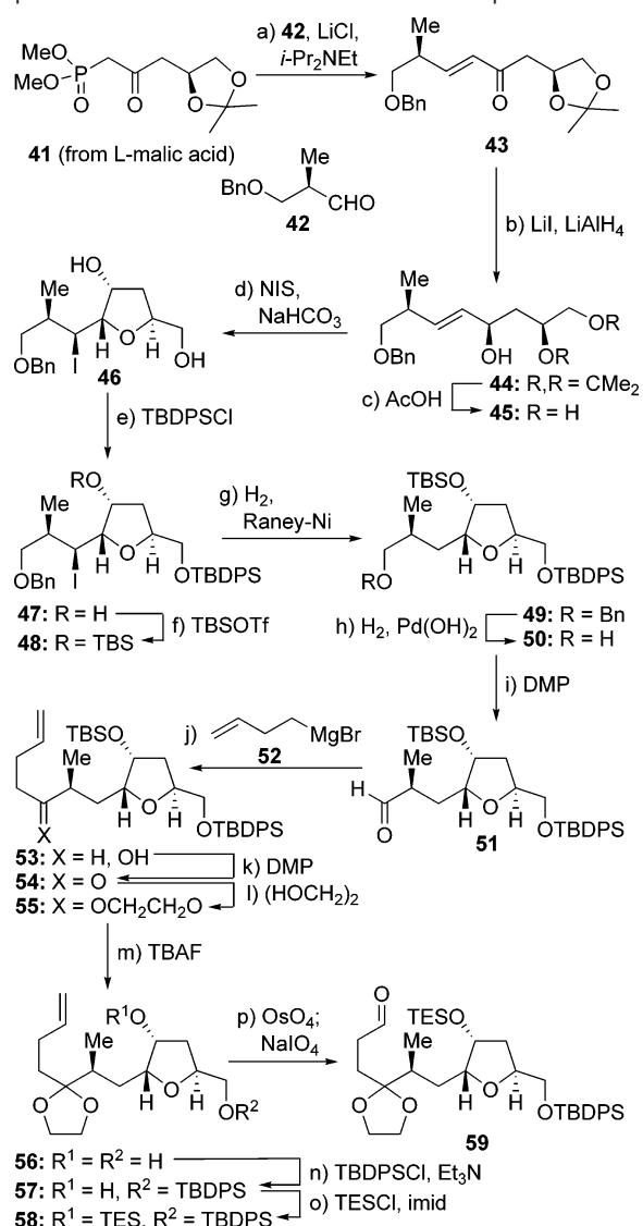
Scheme 5. Synthesis of Aldehyde 59 , a Precursor for the Third Proposed Structure of the ABCD Domain of Azaspiracid-1 9
