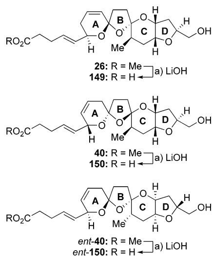
Scheme 12. Synthesis of Truncated Azaspiracid ABCD Analogues 149 , 150 , and ent - 150 a
