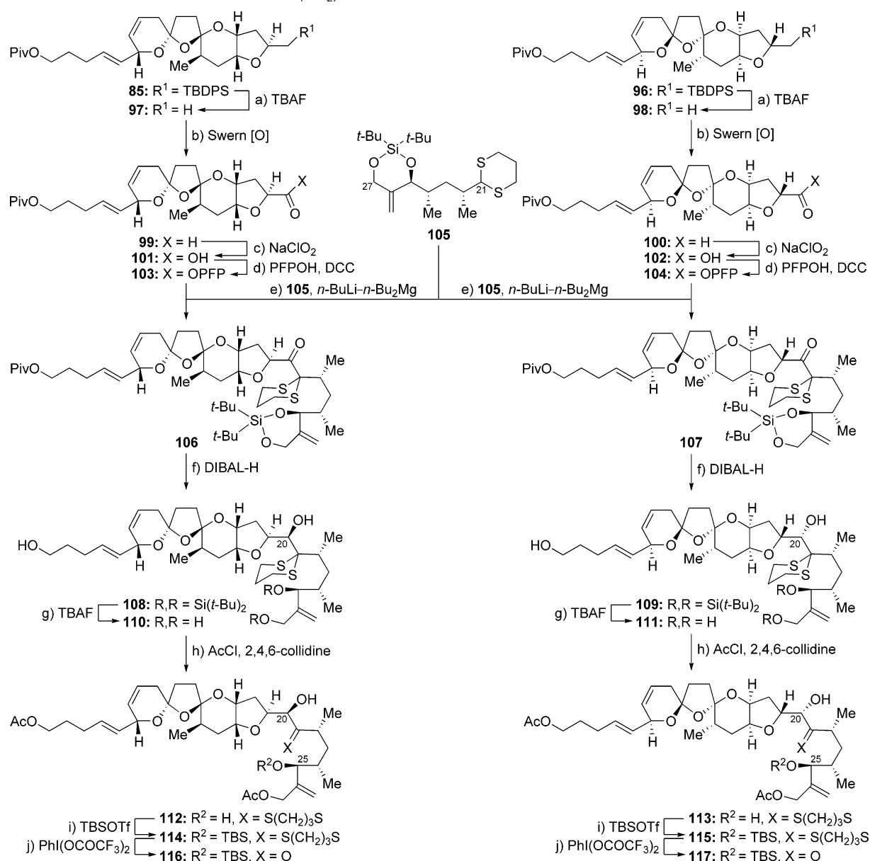
Scheme 8. Construction of the Diastereomeric C 1 –C 27 Advanced Intermediates 116 and 117 a
