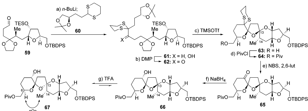
Scheme 6. Cyclization and Epimerization of a Precursor ( 67 ) of the Third Proposed Structure for the ABCD Domain of Azaspiracid-1 a
