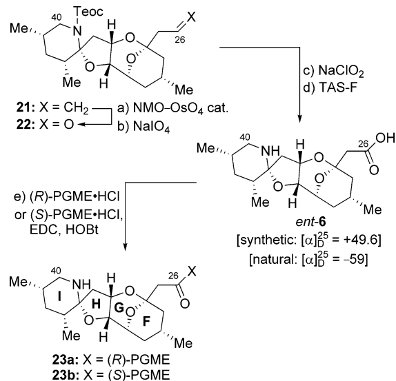
Scheme 2. Synthesis of FGHI Amino Acid ent -6 and Its PGME Derivatives a
