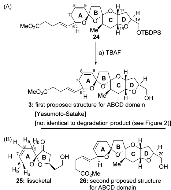
Scheme 3. Synthesis of ABCD Alcohol 3 for Comparison with Degradatively Derived Material (A) and Second Proposed Structure ( 26 ) for the ABCD Domain Based on 1 H NMR Spectroscopic Comparisons with Lissoketal ( 25 ) (B) a
